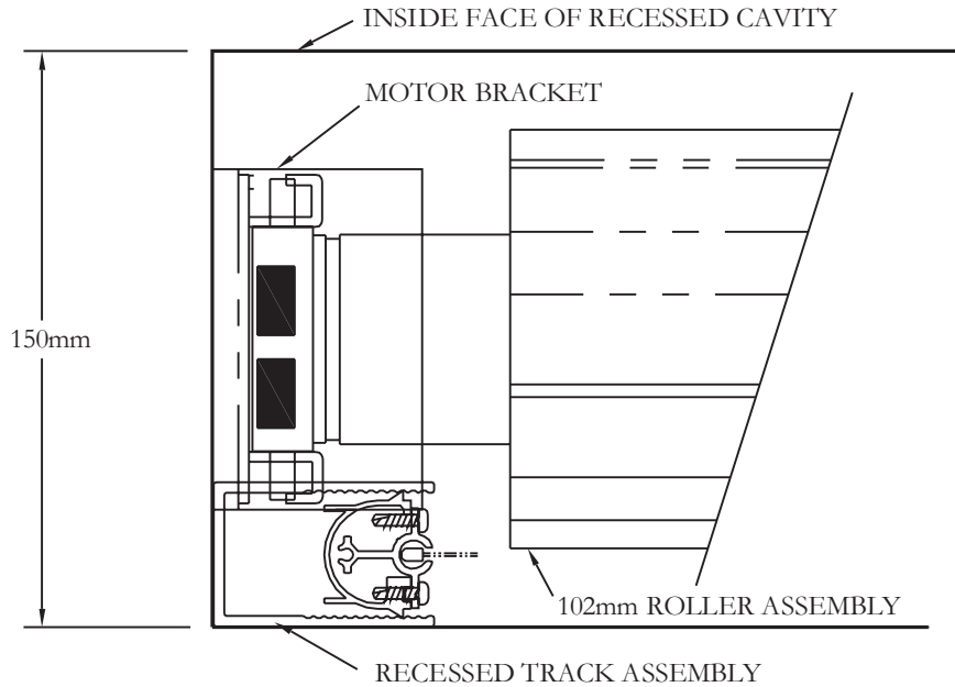
MINIMUM RECESSED CAVITY WITH A 102mm ROLLER
