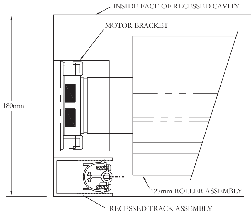
MINIMUM RECESSED CAVITY WITH A 127mm ROLLER
