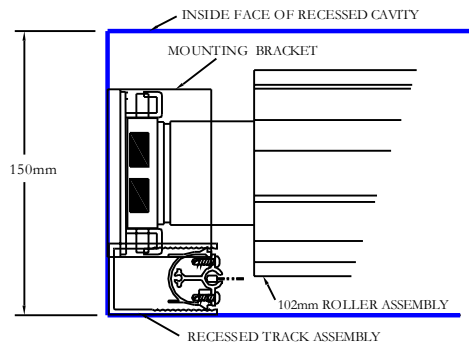
RELATIONSHIP OF U-CHANNEL TO MOTOR BRACKET IN A MINIMUM RECESSED CAVITY C/W 102mm ROLLER
