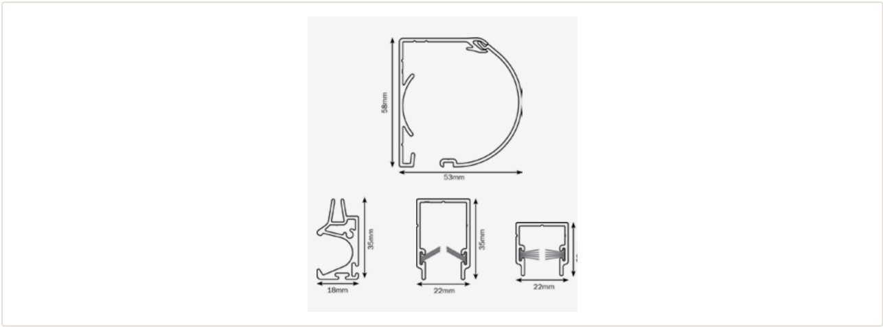
Serene cassette (58 x 53 mm) with side track and sill profiles. Dimensions in millimetres.
