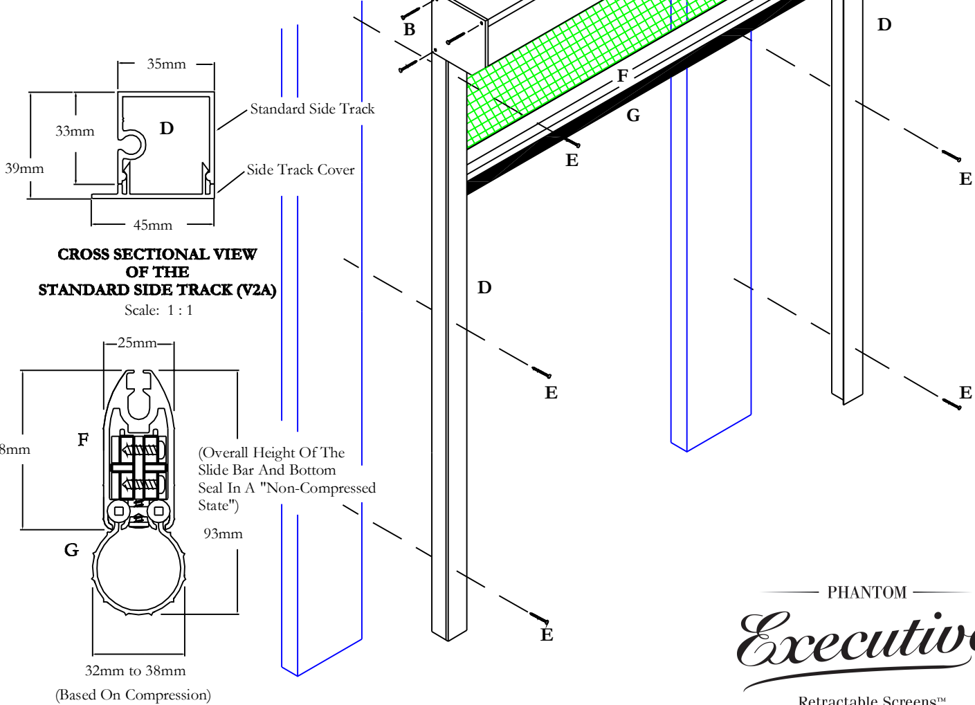
CROSS SECTIONAL VIEW OF THE SLIDE BAR AND 4" BOTTOM SEAL
